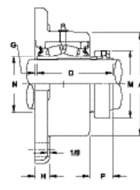
Side View Flange Block
