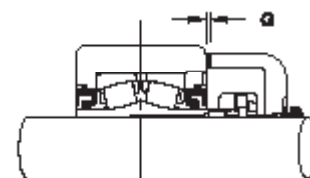
Gasket Thickness
