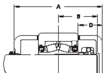
"B" Prefix (1 Open 1 Closed Caps) Example: BMA215
