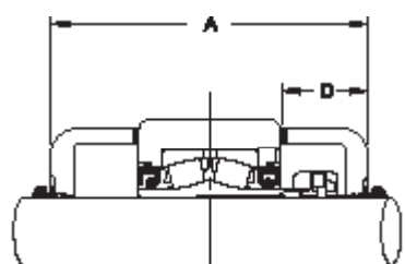
"A" Prefix (Two Open Caps) Example: AMA215
