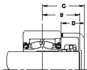
"B" SUFFIX (One Closed Cap) Example: MA215B
