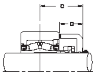
"A" SUFFIX (One Open Cap) Example: MA215A
